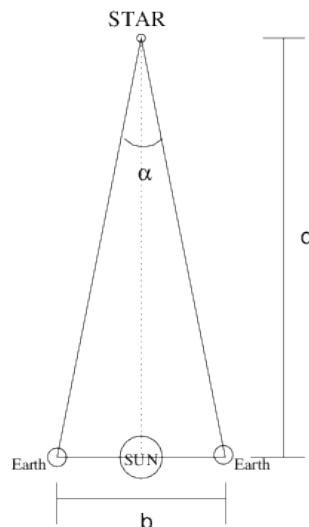
Figure 6.2: Parallax Method for Distance to a Star
