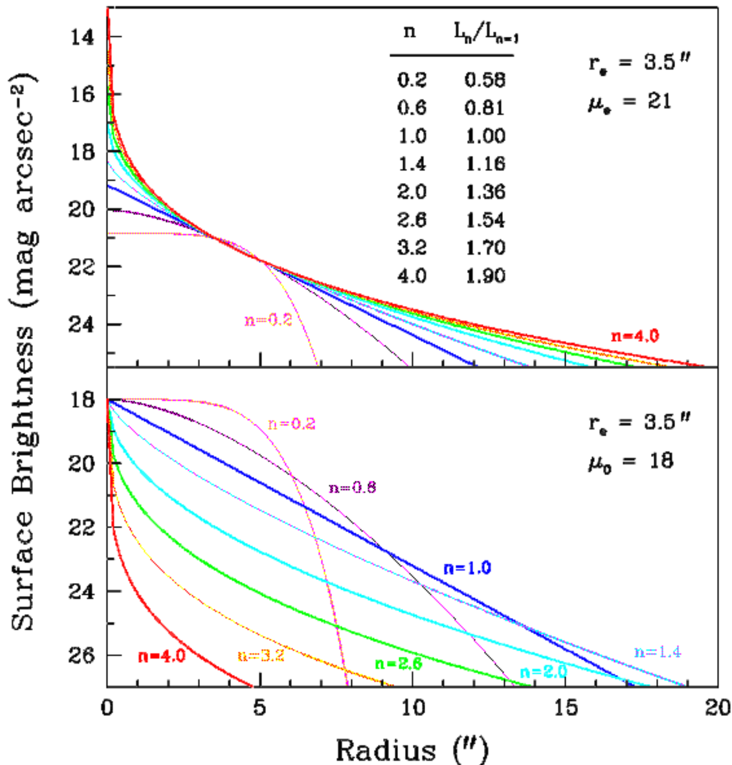
Fig. 2.— Sérsic n profiles for different values of n . The top panel shows profiles with \mu_e = 21 mag arcsec ^{-2} and r_e = 3.5'' for values of n in the range 0.2 < n < 4 . The table lists the relative light contributions of the different profiles normalized to the n = 1 case. The bottom panel shows the same profiles except for a constant CSB of \mu_0 = 18 mag arcsec ^{-2} .
