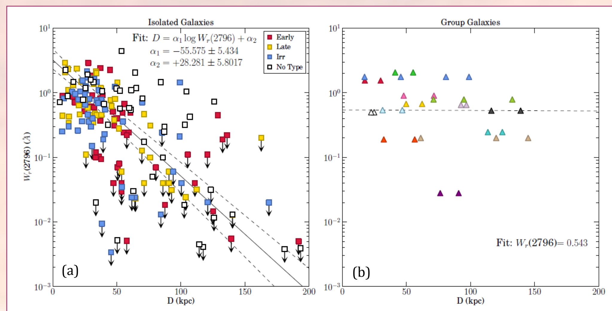
Figure 4 Absorption Line Strength vs Impact Parameter (a) Isolated galaxies. Galaxy types are represented by colors (see legend). The solid line is a log-linear maximum likelihood fit to the data and the dashed curves provide 1\sigma uncertainties. (b) Group galaxies. Different point colors represent different groups. The dashed line is a linear fit consistent with a null slope, showing no anti-correlation with D .
