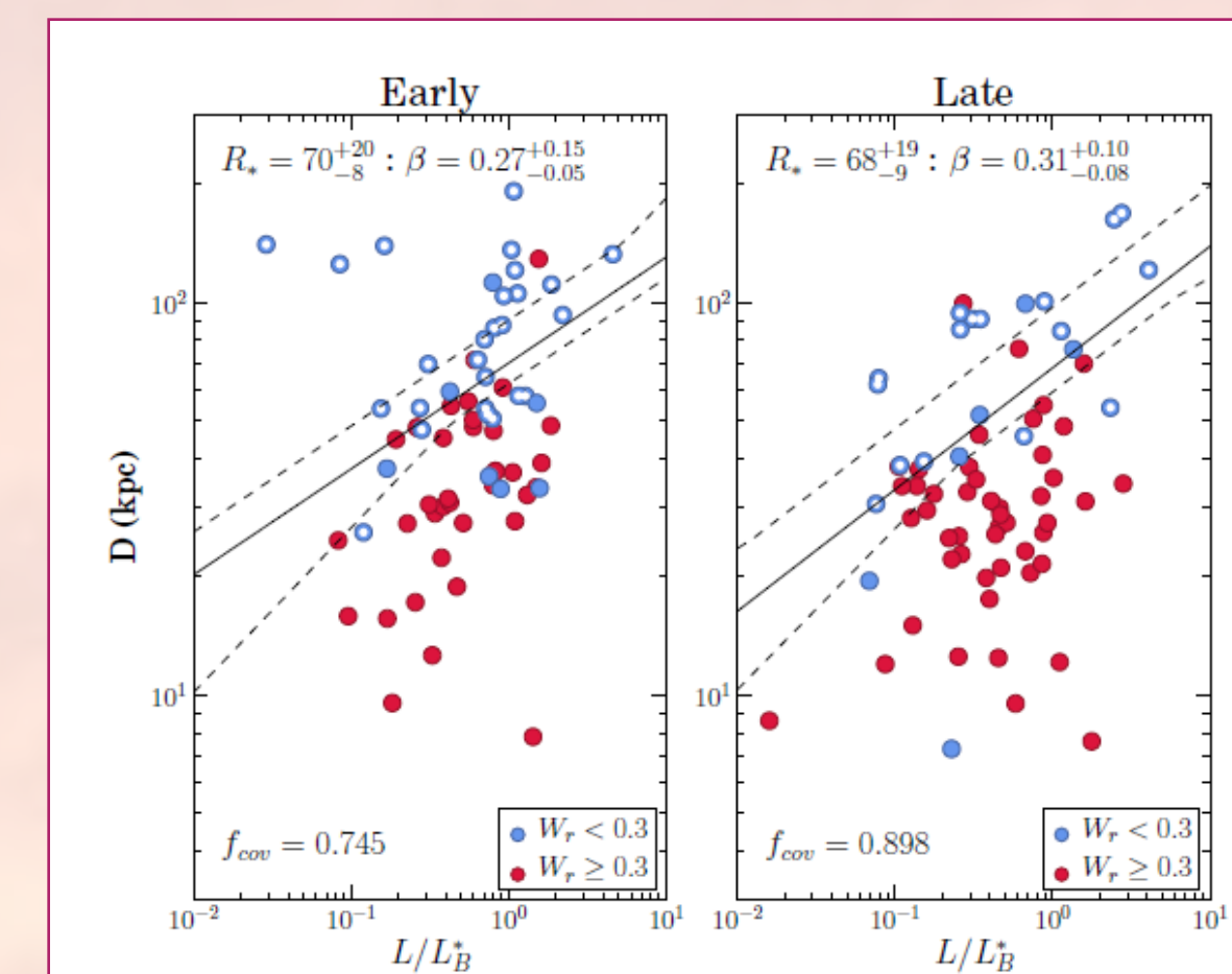
Figure 7 Impact Parameter vs Luminosity for Early and Late Type Galaxies Open points represent galaxies which have limits for W_r(2796) .
