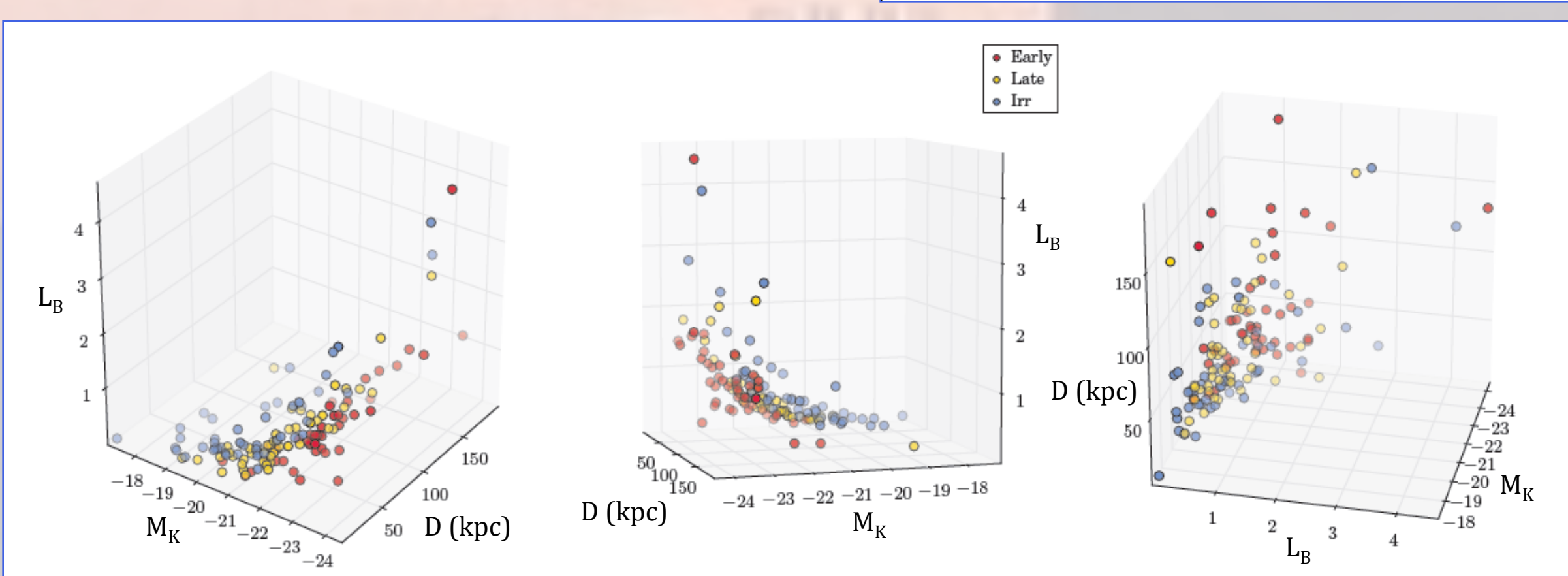
Figure 2 Distribution of the Sample The sample is shown in three different orientations for L_B vs M_K vs D . Data points are color coded by galaxy type (see legend). Only galaxies with measured colors are plotted.
