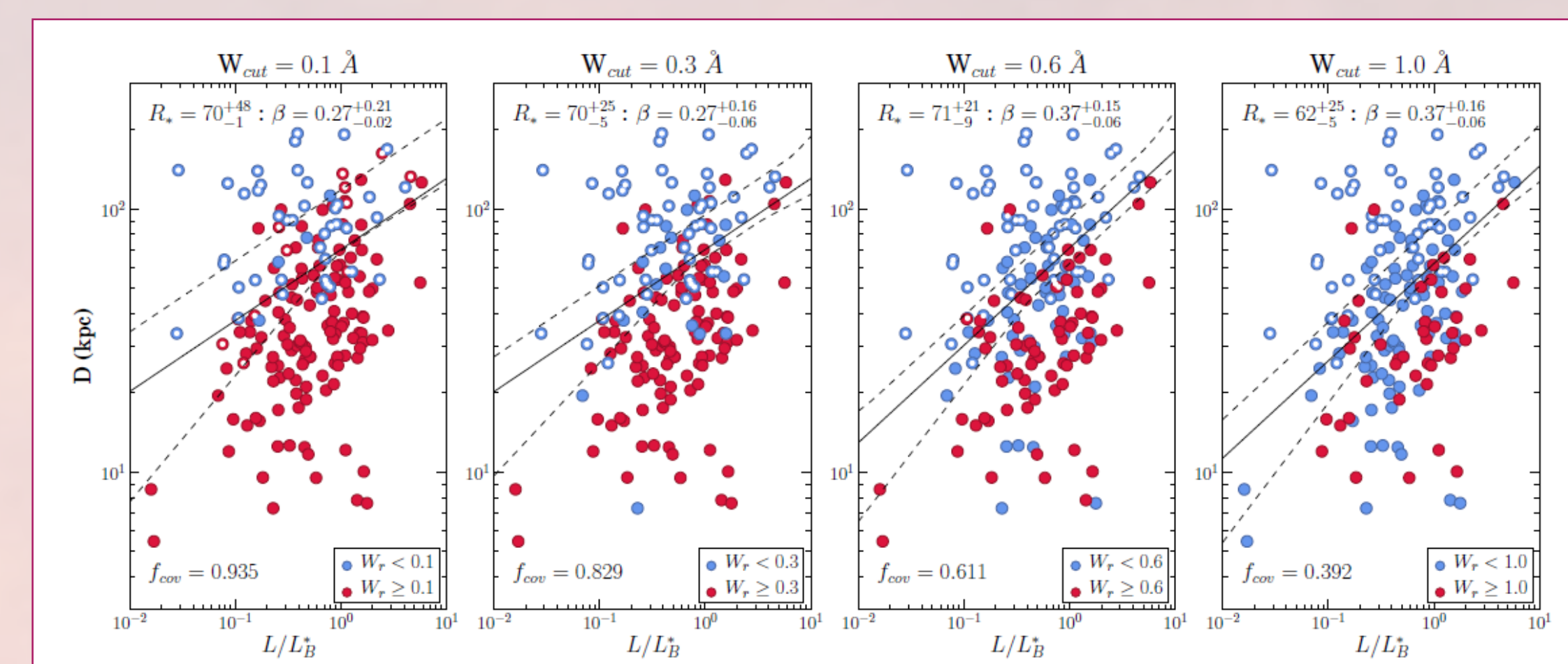
Figure 6 Impact Parameter vs Luminosity for Different W_r(2796) Bifurcations In each panel, blue points are galaxies that have a measured W_r(2796) < W_{\text{cut}} and red points are galaxies with W_r(2796) \geq W_{\text{cut}} . Open points represent galaxies which have limits for W_r(2796) . R_* and \beta give the fit parameters and f_{\text{cov}} gives the covering fraction for each bifurcation. Dashed lines provide the 1\sigma uncertainties in the fit.
