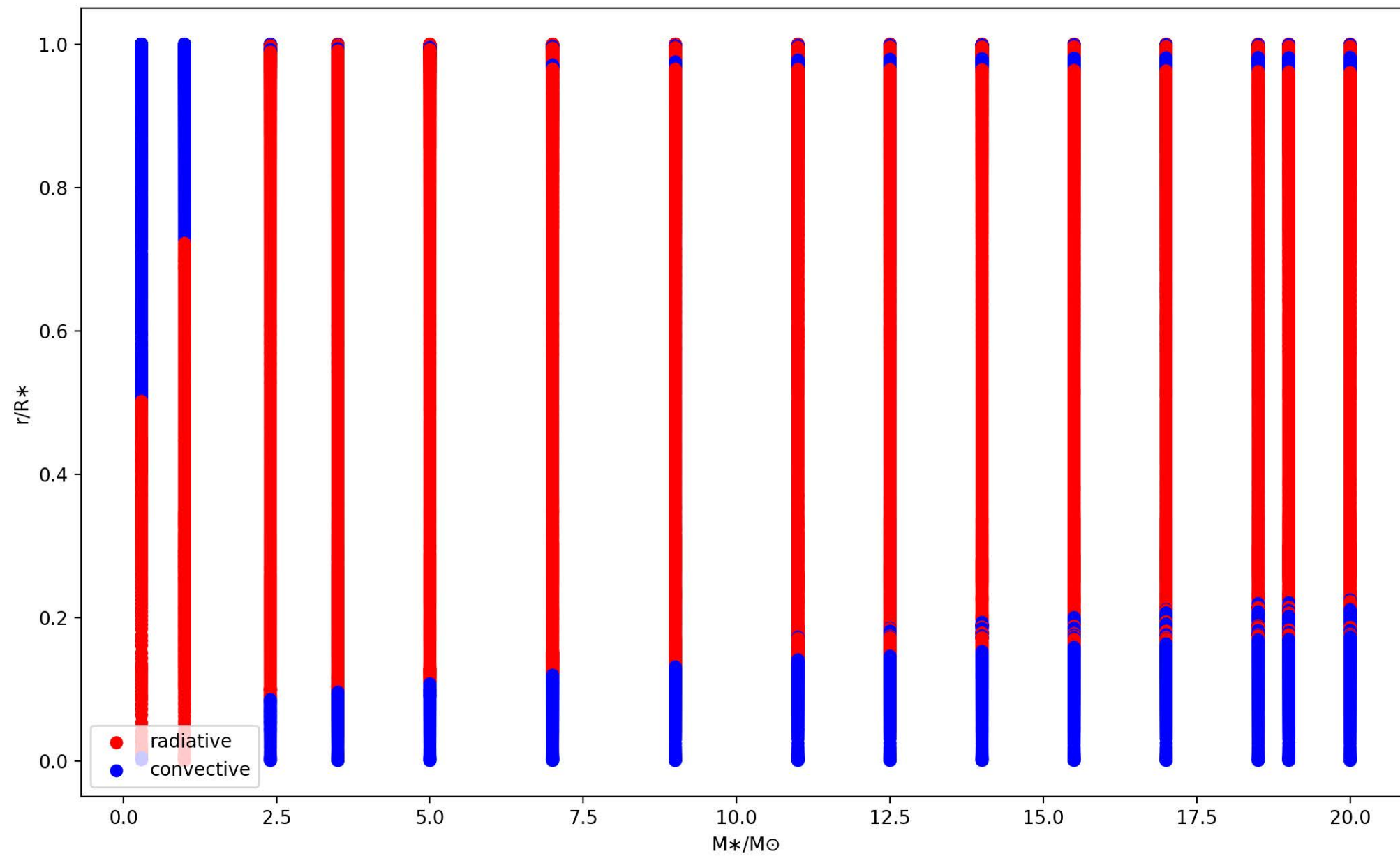
Radiative and convective zone
