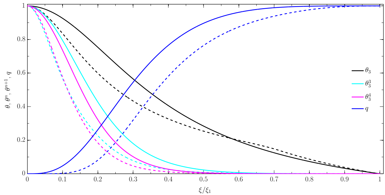
Figure 10.1: Various quantities for a n = 3 polytrope compared to Model S. For each colored curve the solid line is the polytropic solution, and the dashed line is the model Sun.
