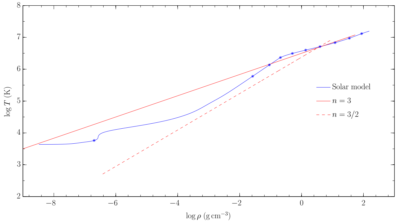
Figure 10.2: A modern solar model compared to 2 different polytropic models. The blue dots on the solar model denote the interior radial coordinate from r = (0.1 - 1.0)R_{\odot} in steps of 0.1. This particular solar model goes slightly beyond the photosphere.
