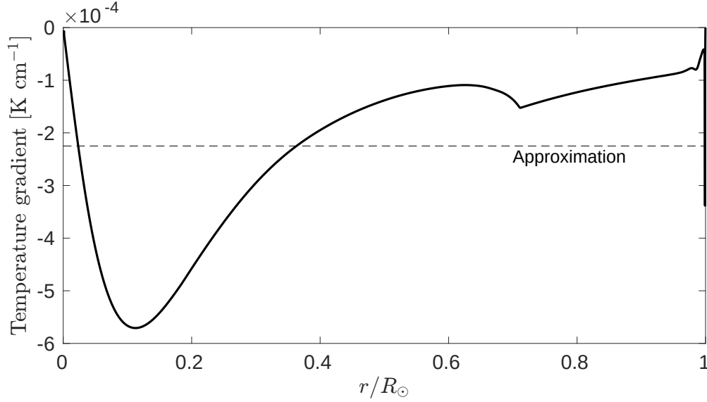
Figure 13.1: The interior temperature gradient of a solar model. Also plotted is a simple estimate of the gradient \sim T_c/R_\odot .
