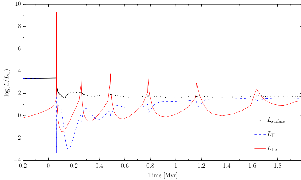
Figure 21.4: Helium flash for a 1M_{\odot} model. Time has been shifted to approximately the start of the flash, which corresponded to about 12 billion years. Note the decrease in the surface luminosity due to the expansion of the He core and cooling of H-burning shell.
