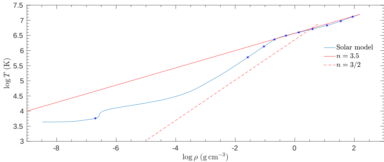
Figure 10.2: A modern solar model compared to 2 different polytropic models. The blue dots on the solar model denote the interior radial coordinate from r = (0.1 - 1.0)R_{\odot} in steps of 0.1. This particular solar model goes slightly beyond the photosphere.
