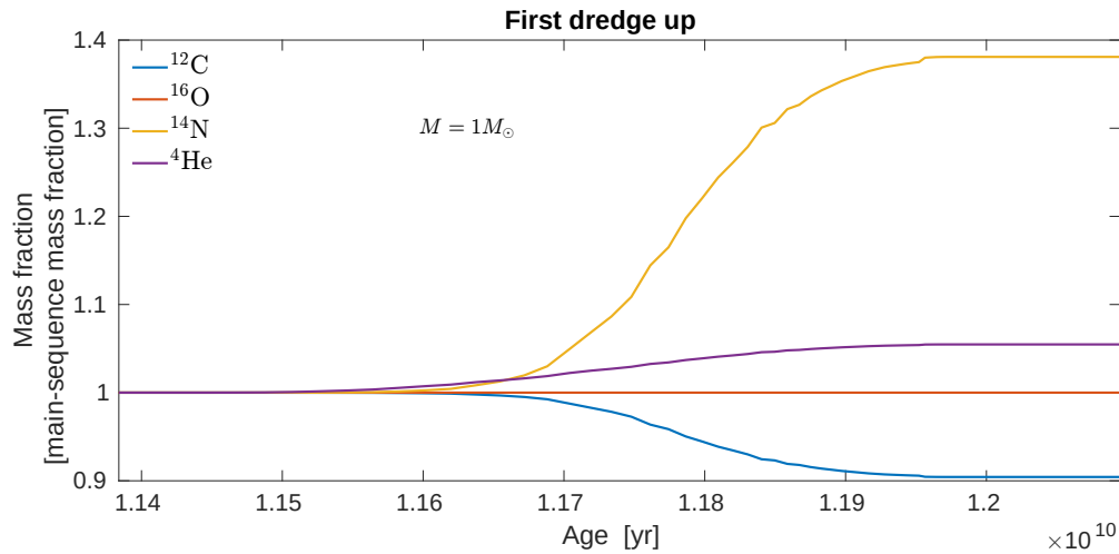
Figure 21.2: Abundance changes at the surface during the first dredge up on the RGB for a solar-mass model.
