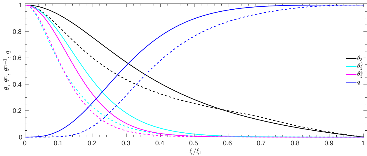
Figure 10.1: Various quantities for a n = 3 polytrope compared to Model S. For each colored curve the solid line is the polytropic solution, and the dashed line is the model Sun.
