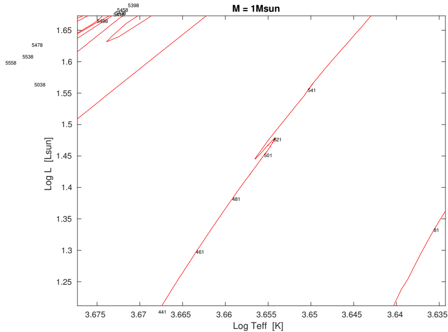
Figure 21.3: A zoom in on the H-R track of the 1 M_{\odot} model during the RGB luminosity bump. The model numbers are annotated.
