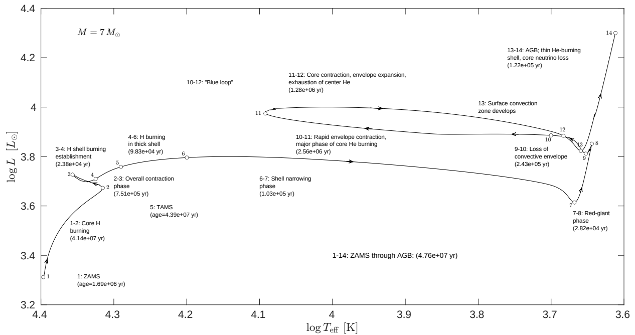
Figure 18.2: Evolutionary track of a 7 M_{\odot} model from the zero-age main sequence to the end of the asymptotic giant branch phase.
