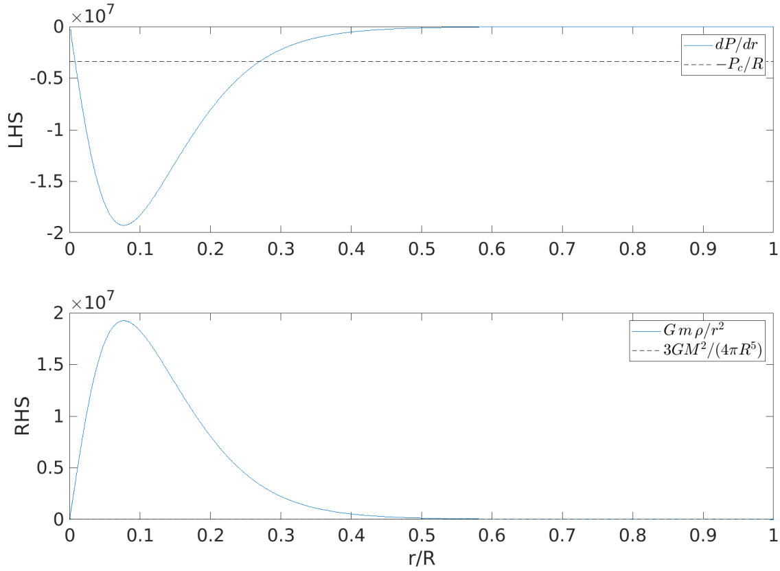
Figure 9.2: Illustration of the approximation made in the example where make simple substitutions.
