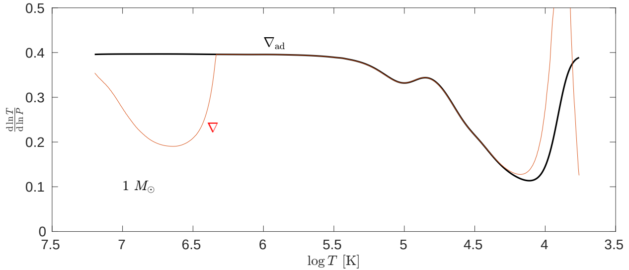
Figure 16.1: The adiabatic temperature gradient of a solar-like model. Note the decrease in the outer layers. Also shown is the true temperature gradient in the model.
