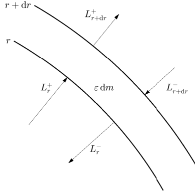
Figure 1.1: Representation of an infinitesimal shell at radius r in a stellar interior. L denotes the luminosity moving toward the surface (+) or toward the center (−).
