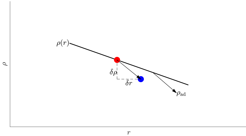
Figure 15.2: Convective instability. The curve \rho(r) denotes the density gradient in some small region of a stellar interior. The arrow is the direction of an adiabat for this material. Take a parcel (red dot) in equilibrium with density \rho , and displace it upwards ( \delta r > 0 ) adiabatically. It ends up where the blue dot is. This parcel now has a lower density than the surroundings ( \delta\rho < 0 ), and so will continue to rise toward the surface until the conditions change (if they change). The density does not decrease sufficiently fast enough to be stable to convection.
