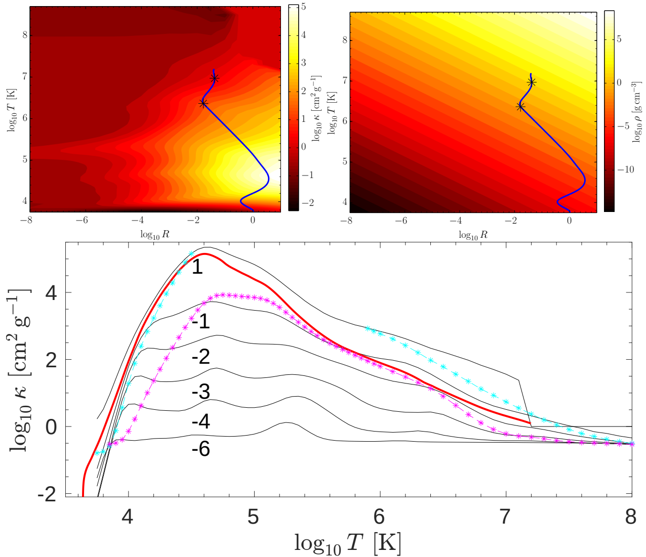
Figure 14.2: (Left top): OPAL Rosseland mean opacity data for a solar composition mixture. The x -axis quantity, R , is defined as R = \rho T_6^{-3} , where T_6 = T \times 10^{-6} as usual. Since R can be multivalued for any \rho, T pair, on the right panel is plotted the density, for reference. In each case the blue curve are the values for a standard interior solar model, and the 2 black stars represent the boundaries of the core and convection zone ( 0.2R_{\odot} and 0.7R_{\odot} , respectively). The direction of increasing T is toward the stellar center. (Bottom): Cuts through the opacity values for specific values of \log R , given by the labeled curves. The red curve is the opacity from a current solar model. The cyan and the magenta symbols represent the 0.5 and 0.99 ionization curves for pure hydrogen, respectively, as in Figure 12.2. (Specifically the data are from computation 200503120009, Table 73. The calculations consider about 20 species.)
