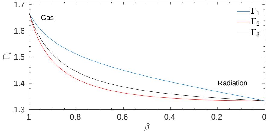
Figure 12.1: The various adiabatic exponents for different mixtures of ideal gas particles and photons.
