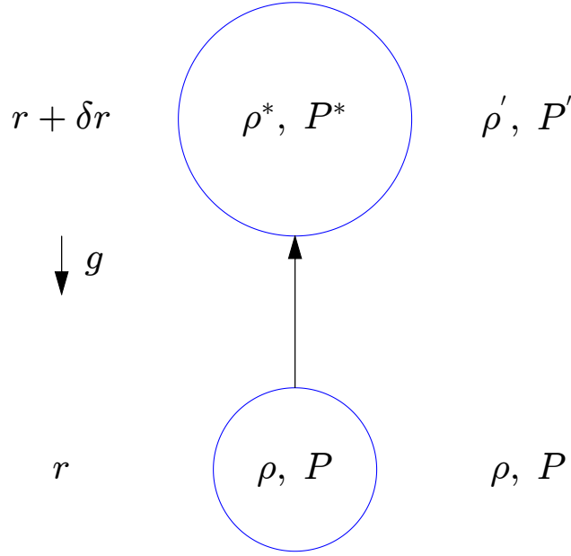
Figure 15.1: A blob is displaced adiabatically from position r upwards to position r + \delta r , against the direction of gravity. What happens next depends on the environmental conditions. Inspired by Christensen-Dalsgaard [2008].
