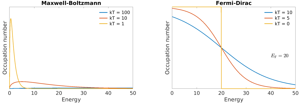
Figure 7.1: Differences in particle behavior depending on the type considered. For Maxwell-Boltzmann, it's easiest to consider Eq. 6.8. As the temperature decreases, the particles want to be in the zero energy state. For higher temperatures, the peak occupation numbers are at higher temperatures. For fermions, at T = 0 , all states are filled by 1 particle up to the (arbitrarily chosen here) Fermi energy. Temperatures are given in energy units k_B T .
