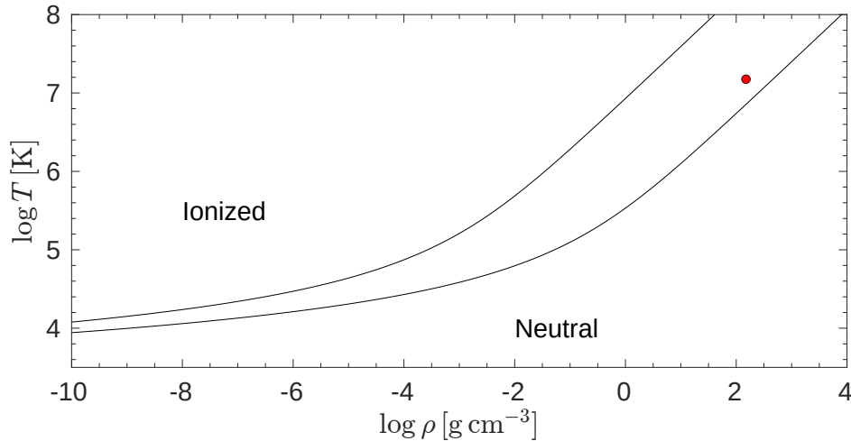
Figure 12.2: Ionization of a pure H gas using Equation (12.19). The lower line represents the state at 50% ionization, while the upper is for 99%. The red dot shows the conditions in the Sun's core, which corresponds here to about 70 % ionization.
