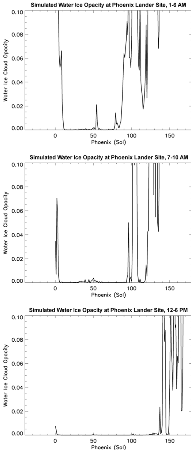
Figure 4. (top) Simulated water ice opacity over the lander site for 0100–0600 LT, (middle) 0700–1000 LT, and (bottom) 1200–1800 LT. Morning clouds begin on sol ~90. As the season progresses, clouds extend later into the morning hours. No clouds are seen in the afternoon hours until the very end of the mission.
