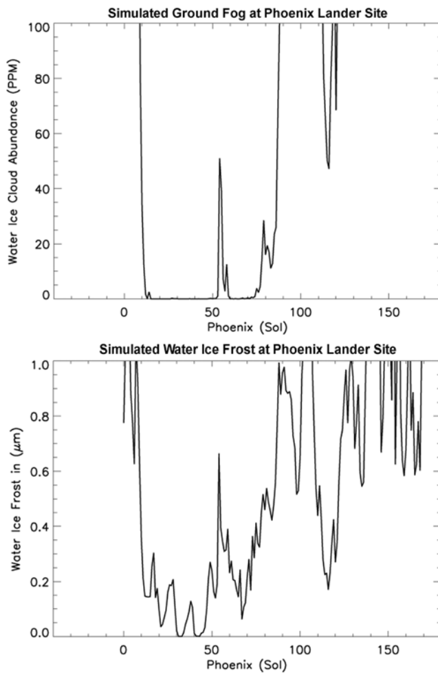
Figure 6. (top) Simulated ground fog formation over the Phoenix site in ppm (0100–0600 LT) and (bottom) daily frost accumulation in \mu\text{m} . The GCM accounts for both water ice cloud precipitation and direct deposition of frost onto the ground. The dramatic increase in ground frost correlates with the sudden and short-lived appearance of a ground fog in the GCM between sols 50 and 60.
