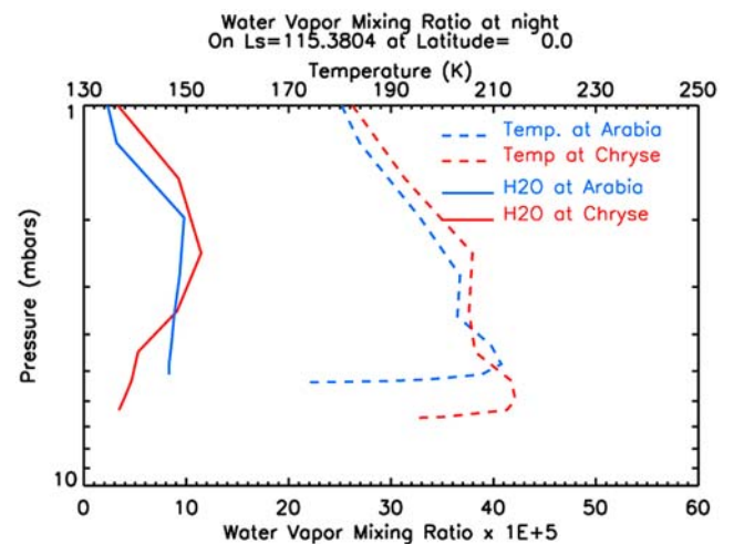
Figure 9. Simulated nighttime (0000–0600 LT mean) vertical water vapor mixing ratio and temperature profile for a location of preferred deposition (Arabia; 0^\circ\text{N} , 18^\circ\text{E} ) and desiccation (Chryse; 0^\circ\text{N} , -30^\circ\text{E} ). The offset in pressure is due to a 2 km change in elevation between the two locations. Arabia is 20 K colder and is threefold wetter, making condensation more likely than in Chryse.
