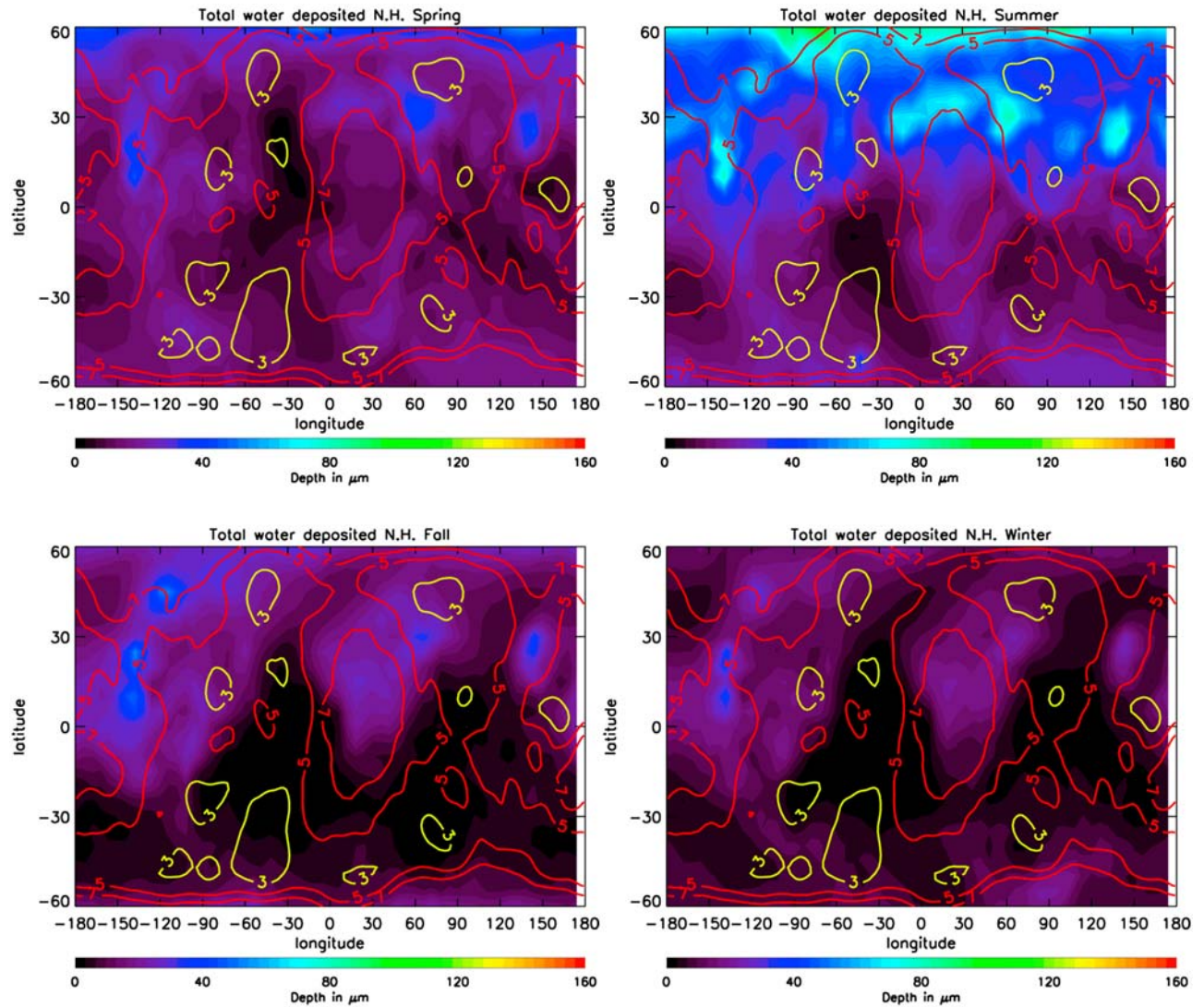
Figure 6. These plots represent the total integrated water ice deposited (precipitation and direct deposition) by season in the model. The contour lines represent 3%, 5%, and 7% by mass observed WEH [Feldman et al. , 2004a].
