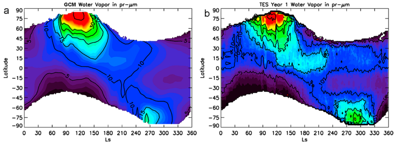
Figure 3. (a) Model-derived zonal mean water vapor abundances in \text{pr } \mu\text{m} . (b) TES-derived abundances [Smith, 2004]. Contours are 5, 10, 15, 20, 25, 30, 50, and 70 \text{pr } \mu\text{m} . The white shading over the poles is where the surface temperatures were too cold for TES to obtain accurate values.
