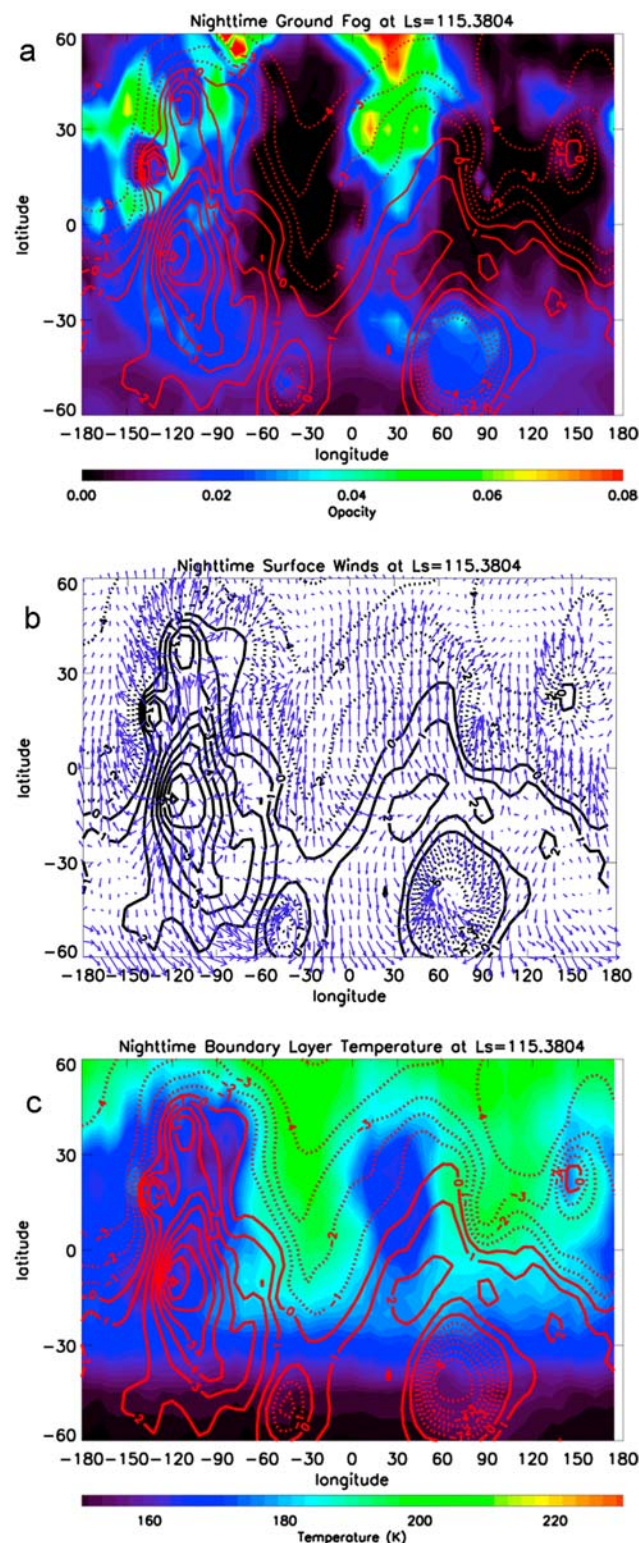
Figure 7. (a) The nighttime (0000–0600 LT mean) near-surface ground fog water ice opacity. The red contour lines represent the underlying topography in km. The season is northern summer ( L_s \sim 115^\circ ). The cloud opacity is solely that contributed by the ground fog. This opacity is calculated only from the surface to a height of \sim 200 m since this is the vertical extent of the ground fog. (b) The direction and relative magnitude of nighttime (0000–0600 LT mean) surface winds during the same season ( L_s \sim 115^\circ ) as the nighttime surface fog. Black contours are surface topography in km. At night, near-surface circulation decouples from the global thermally direct (Hadley) circulation and flows down the slope of the topography. (c) The simulated nighttime (0000–0600 LT mean) atmospheric temperatures in the lowest atmospheric layer for the same season ( L_s \sim 115^\circ ) as Figures 7a and 7b. The red contours are surface topography in km. Local minima occur over Arabia ( 10^\circ N, 20^\circ E), Tharsis ( 15^\circ S, -100^\circ E), and Elysium Mons ( 20^\circ N, 140^\circ E) regions of maximum water ice deposition.
