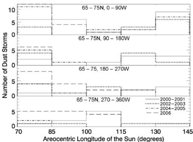
Figure 7. The frequency of dust storm activity observed at Phoenix latitudes in MOC wide-angle observations as a function of L_s , using a bin size of 15^{\circ} of L_s . MOC observations span the late northern spring and midsummer seasons over four consecutive Mars years from November 2000 to October 2006. No distinction between local and regional storms was made.
