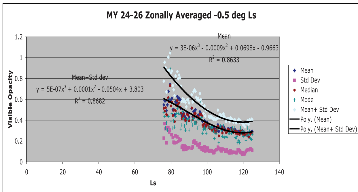
Figure 6. Visible opacity means and standard deviations for three Mars years of TES dust and water-ice opacity data averaged over latitudes of 65^{\circ} – 72^{\circ} N and by 0.5 L_s ( \sim 1 sol). A third-order polynomial was fit to the mean values and to the mean plus standard deviation values.
