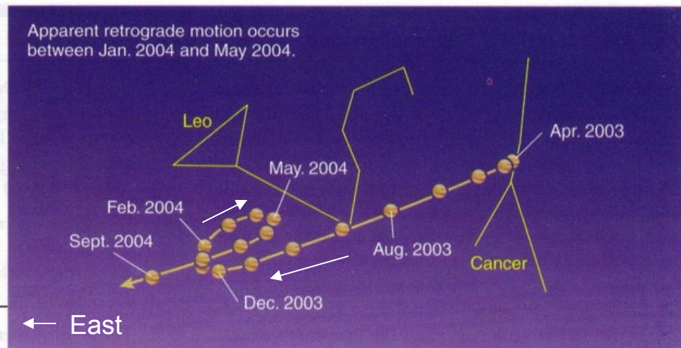
Dots represent Jupiter's approximate position at 1-month intervals. (Jupiter not to scale.)
