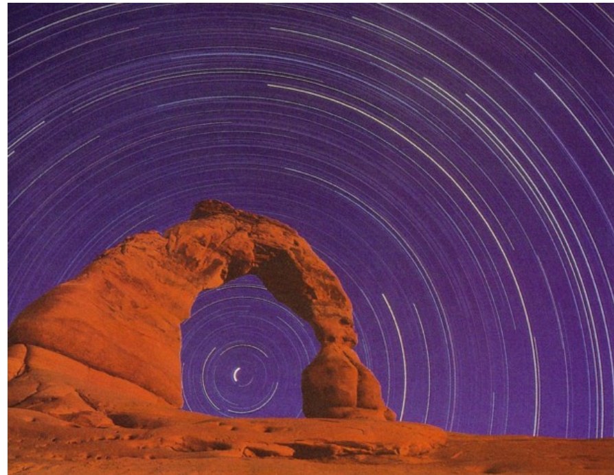
Star trails – 6 hour exposure
