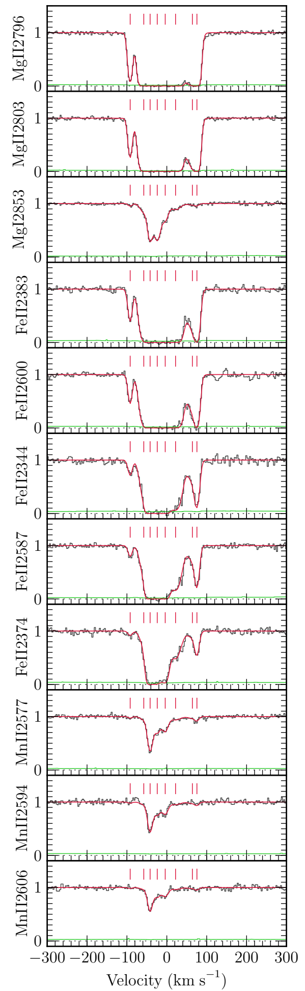
J010054 + 021136, z_{\text{abs}} = 0.612586
