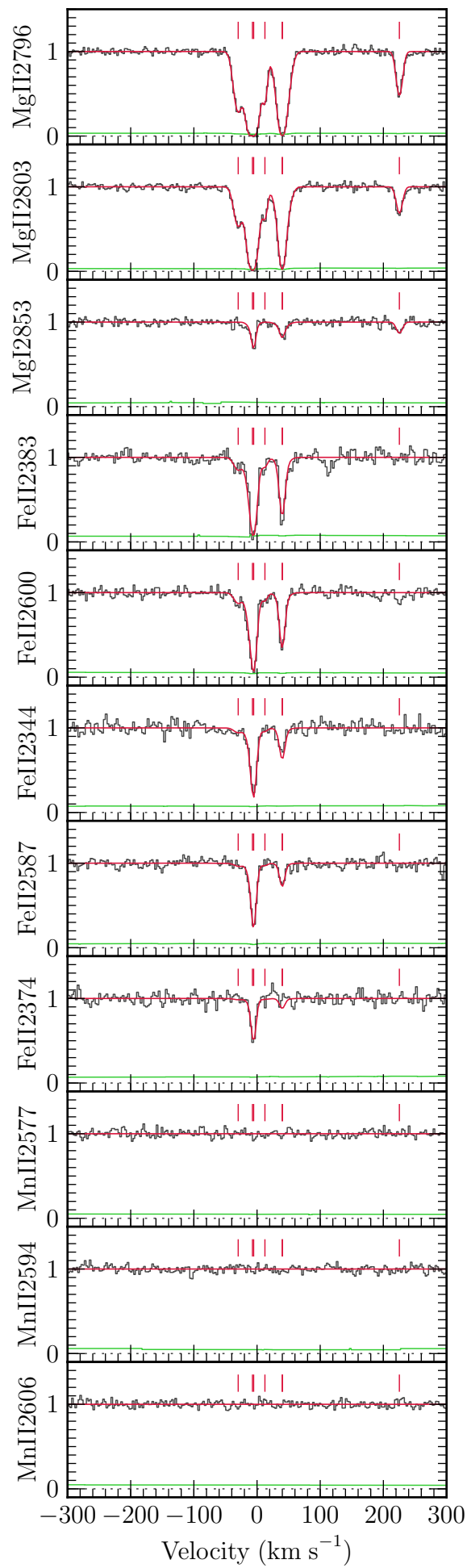
J125048 + 395140, z_{\text{abs}} = 0.772957
