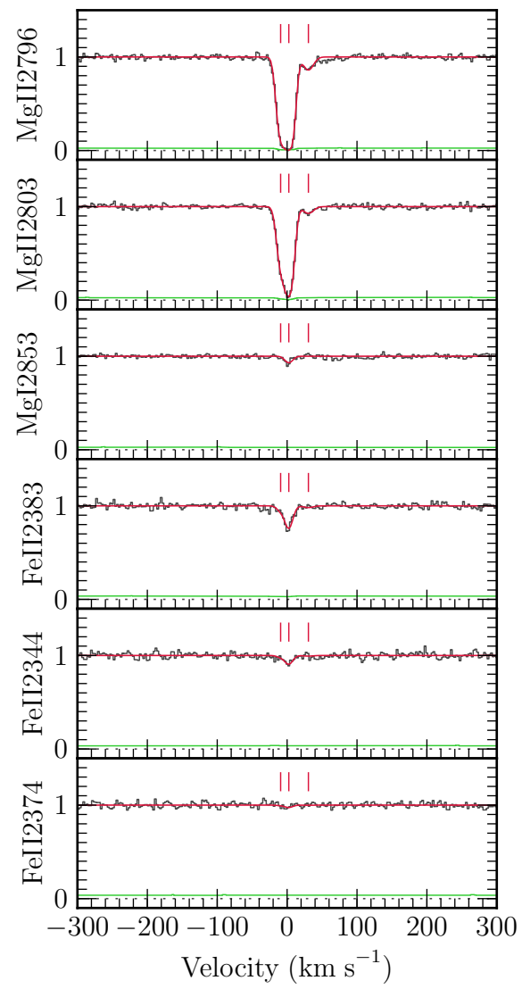
J123200 - 022405, z_{\text{abs}} = 0.756903
