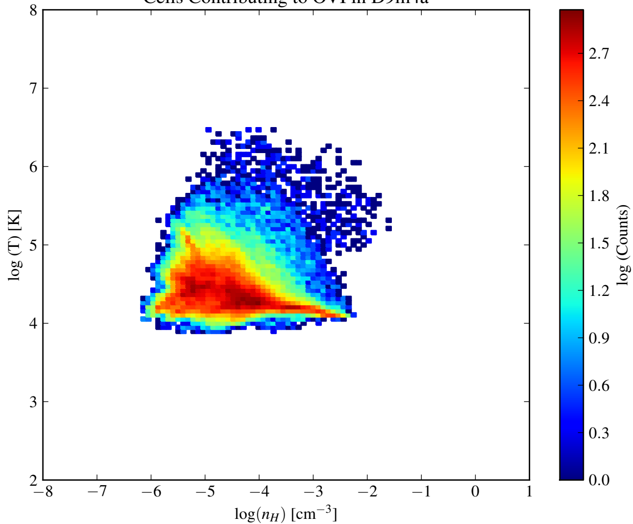
Cells Contributing to OVI in D9m4a
