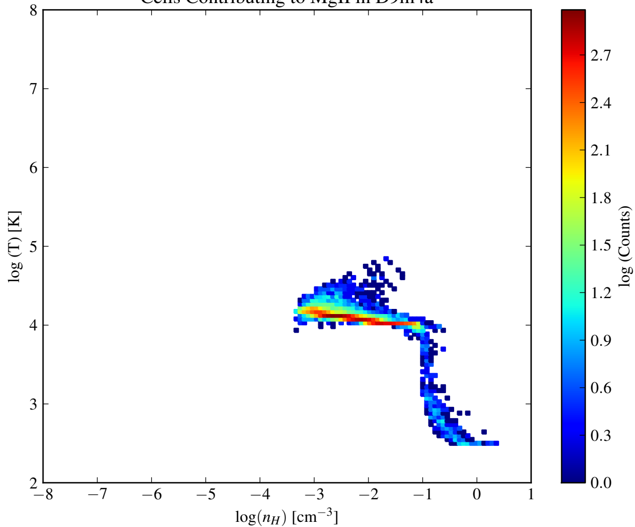
Cells Contributing to MgII in D9m4a
