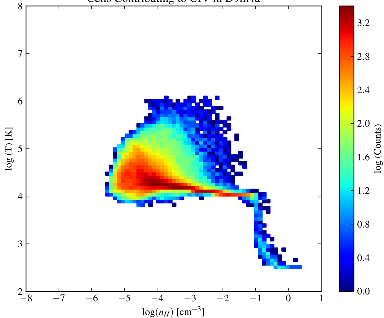
Cells Contributing to CIV in D9m4a
