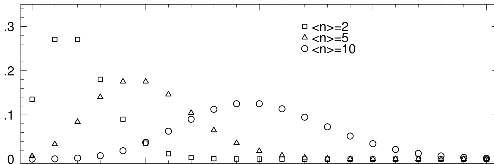
f(n, \langle n \rangle) , Poisson Distribution
