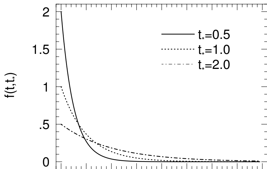
Exponential Distribution
