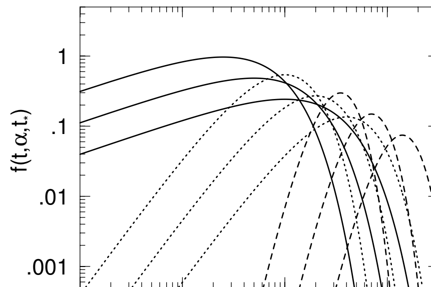
Gamma Distribution
