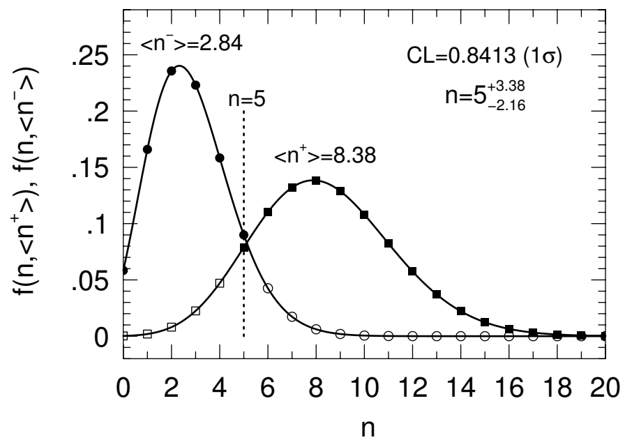
(b) 1\sigma Poisson Distributions ( n=5 )
