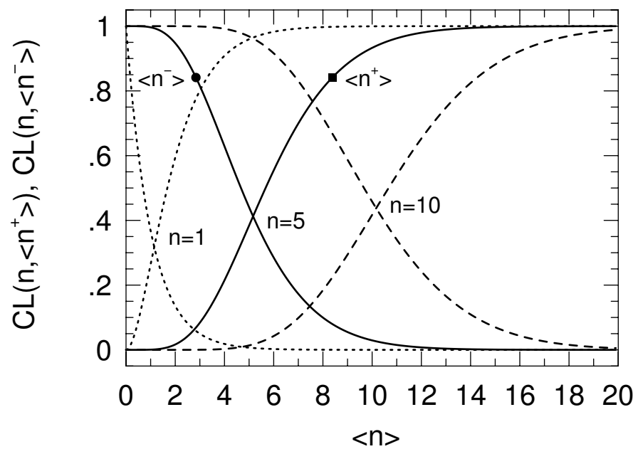
(a) Poisson Confidence Levels
