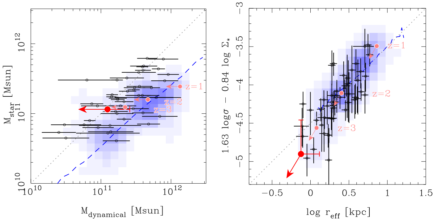
Figure 5. Left: stellar mass plotted against dynamical mass. The dotted line shows M = M_{\text{dyn}} . The black points are the lower redshift objects ( z \sim 2 ) as in Figure 4. The shades are quiescent galaxies from LEGA-C, and the dashed curve is the running median of the distribution of quiescent galaxies with \text{sSFR} < 10^{-10} M_{\odot} \text{ yr}^{-1} drawn from SDSS DR15 (Aguado et al. 2019). SFR and stellar mass are from Granada FSPS (Ahn et al. 2014). The red point is the z = 4 object. The pink points are the expected evolutionary track assuming constant velocity dispersion (see the text for details). Right: mass fundamental plane. The dotted line is a fit from Bezanson et al. (2013). The other symbols are the same as those in the left panel.
