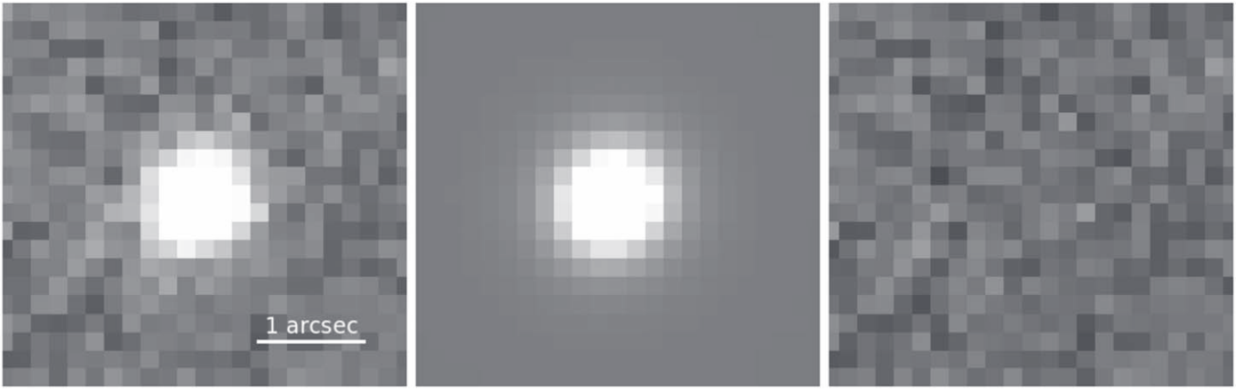
Figure 3. Panels show the i -band image from HSC, the best-fit model, and residual, from left to right. The flux scales are the same in all the panels.
