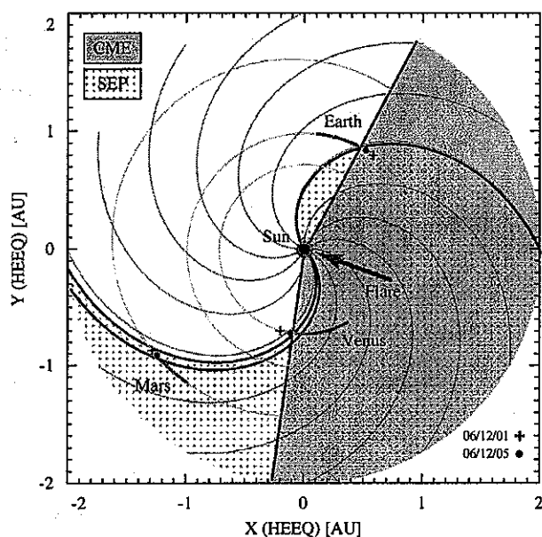
Fig. 1. The locations of Venus, the Earth and Mars relative to the Sun in December 2006. The location of the flare of December 5 is indicated by an arrow. The solid curves are the magnetic field lines of the ideal Parker spiral. Shaded and hatched areas indicate the regime deduced to be affected by CMEs and SEPs originating in active region 930 (see text for details). These areas are deduced from available data at Earth, Venus and Mars; therefore, the affected areas are expected to be wider than those shown in the figure.
