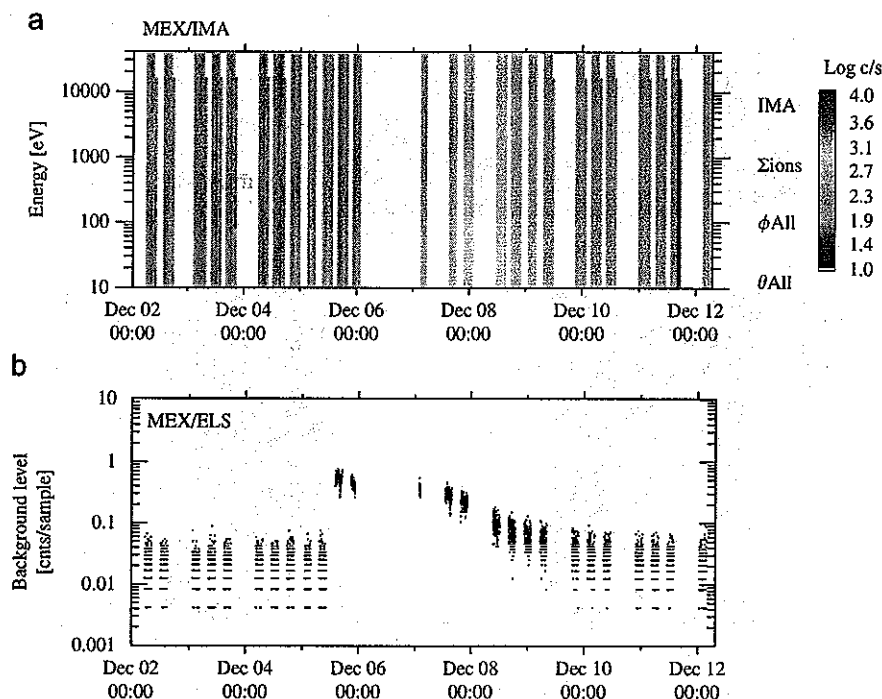
Fig. 3. (a) The energy-time spectrogram obtained from ASPERA-3/IMA and (b) a total count rate in the highest 15 energy steps of ASPERA-3/ELS (a proxy for background level) on board Mars Express between December 2 and 12, 2006.
