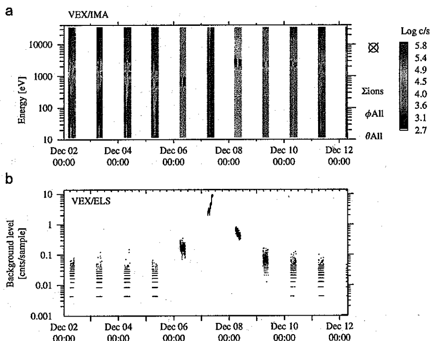
Fig. 2. (a) The observed energy–time spectrogram from ASPERA-4/IMA and (b) a total count rate in the highest 15 energy steps of ASPERA-4/ELS (a proxy for background level) on board VEX between December 2 and 12, 2006.
