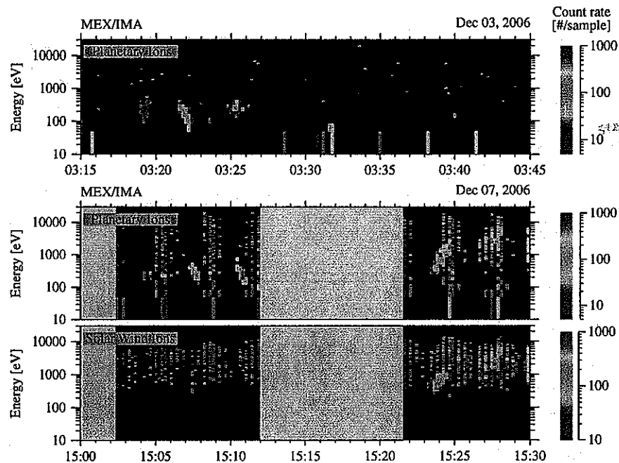
Fig. 4. Energy–time spectra of escaping ions inside the induced magnetosphere boundary recorded by MEX/IMA before the solar flare happened (on December 3, 2006, top panel) and during the SEP event (on December 7, 2006, middle panel). The energy–time spectrum for solar wind protons on December 7, 2006, is shown in the bottom panel. Background counts have been subtracted. Due to high background counts, onboard memory overflowed and data have been lost between 14:56–15:02 UT and 15:12–15:22 UT.
