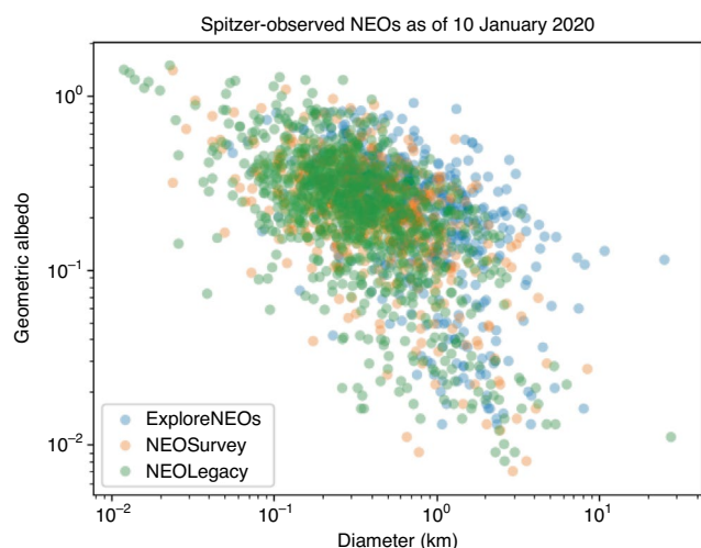
Fig. 1 | Composite albedo and diameter results for the Spitzer NEO surveys (2,204 unique objects). Overall, the uncertainty on any given solution of diameter and albedo is relatively large ( \pm 20\% and up to \pm 50\% , respectively 7,8 ), but the size and albedo distribution properties of the NEO population as a whole can be derived given the large number statistics. There is a clear bias against the smallest, darkest (that is, lowest albedo) NEOs, because the observed samples were chosen from optically detected NEOs.
