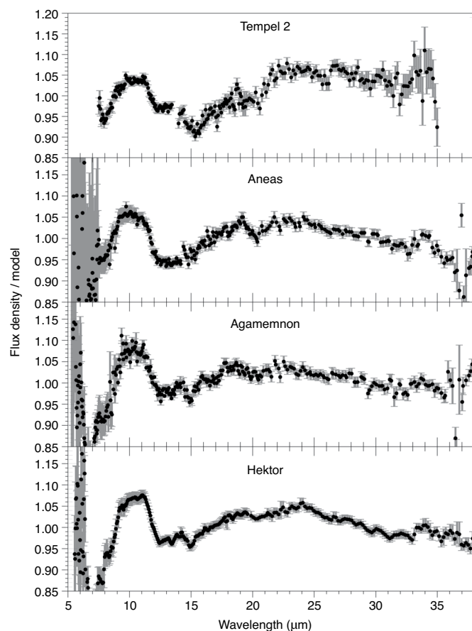
Fig. 2 | Spitzer/IRS spectra of three Jovian D-type Trojans. Emissivity—calculated as flux density divided by a thermal model—for (1172) Aeneas, (911) Agamemnon and (624) Hektor (from ref. 17 ), as compared to the nucleus of comet 10P/Tempel 2 (ref. 66 ). The spectra are very similar and all show 9–12, 18–20 and 34 \mu\text{m} features indicative of fine-grained ferromagnesian olivine and pyroxene silicates, similar to features seen in cometary coma dust spectra. Figure reproduced with permission from ref. 66 , Elsevier.
