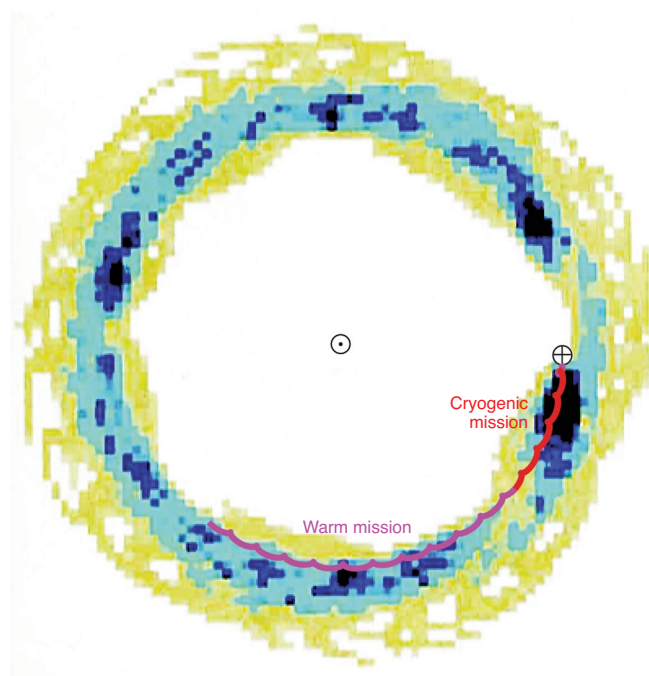
Fig. 3 | Model of the Earth's dust ring based on Spitzer's measurements around the Earth's orbit. Spitzer's observations showed that a ring of dust from comet tails and broken asteroids follows the Earth in its orbit. A broad cloud of these >20 \mu\text{m} particles, about seven million miles wide, trails behind the Earth at about 80 times the Earth–Moon distance. Yellow, blue and black colours show low to high resonant ring dust density. Spitzer's orbital path relative to Earth is shown as the red and purple curve, with the cryogenic and warm mission periods labelled. Figure adapted with permission from ref. 36 , Elsevier.
