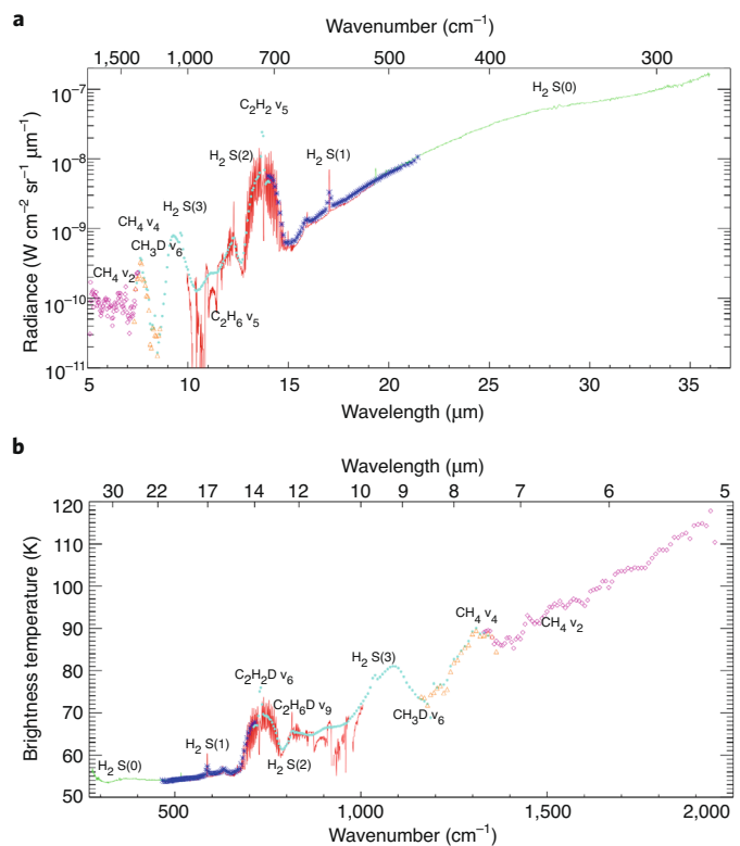
Fig. 6 | Disk integrated spectrum of Uranus. a , Radiance as a function of wavelength (bottom axis) and wavenumber (top axis). b , Equivalent brightness temperature as a function of wavenumber (bottom axis) and wavelength (upper axis). Some spectral features are identified for clarity in each panel. Different instrument modules are coded in different colours and shapes: SL2 (purple diamonds), SL 'bonus order' (green asterisks), SL1 (light blue points), LL2 (dark blue asterisks), SH (red lines) and LH (green points). (Details on the instrument modules can be found in ref. 51 .) Figure adapted with permission from ref. 51 , Elsevier.
