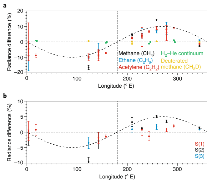
Fig. 5 | Longitudinal variability of Uranus in December 2007. The figure shows the percentage radiance difference from the global average spectrum, along with non-negligible standard errors. a , Significant variations exist for hydrocarbon species present in the stratosphere; the hydrogen-helium continuum and deuterated methane (arising from higher pressures in the troposphere) show considerably less variation. A 10% amplitude sinusoid is shown for reference, but has not been fitted to the sparse data. b , Hydrogen quadrupole measurements, with a 5% amplitude sinusoid displayed for reference (but not fitted). The features labelled as S(1), S(2) and S(3) are the hydrogen quadrupole lines, which are the rotational transitions of hydrogen in the mid- and far-infrared. The S(1) line is at 587\text{ cm}^{-1} ( 17.0\text{ }\mu\text{m} ), S(2) is at 814\text{ cm}^{-1} ( 12.3\text{ }\mu\text{m} ) and S(3) is at 1034\text{ cm}^{-1} ( 9.7\text{ }\mu\text{m} ).
