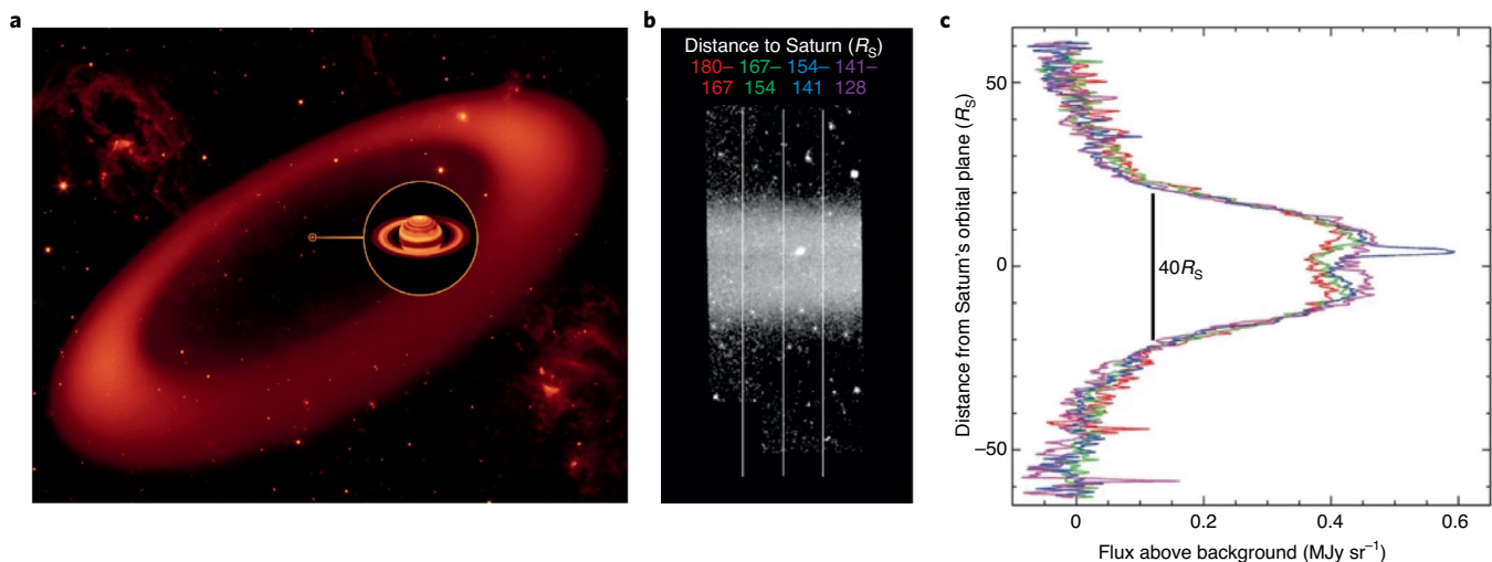
Fig. 4 | Saturn's Phoebe ring. a , Model full-ring image based on the results of Spitzer's MIPS photometric imaging. b , Detail of the 24 \mu\text{m} Spitzer ring imaging, showing the location of three transepts used to extract profile information. The ring is notably diffuse in its interior but has relatively well-defined, sharp boundaries. c , Profile cuts through the ring, showing its relative interior uniformity, minima at and symmetry around Saturn's orbital plane, and edge boundaries. Images reproduced courtesy of NASA/JPL-Caltech/R. Hurt (SSC) ( a ); adapted with permission from ref. 40 , Springer Nature Ltd ( b,c ).
