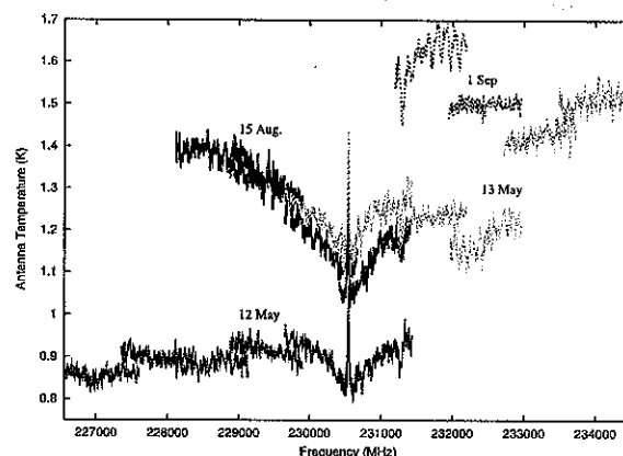
Fig. 1. An overview of all observations. Data are plotted directly in antenna temperatures, i.e. are not corrected for forward and main beam efficiencies, or Neptune's filling factor. Black: Aug. 15, 2003. Blue (dashed line): Sep. 1, 2004. Red: May 12, 2004. Green (dashed line): May 13, 2004. The absorption near 231 280 MHz is due to telluric ozone.
