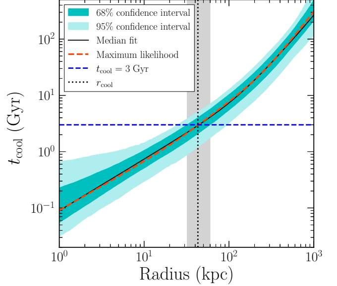
Figure 4. The cooling time profile for SPT0607, computed assuming an isothermal temperature profile and density profiles derived in Section 3.1.2. The radius corresponding to t_{\text{cool}} = 3 Gyr is shown with a black dotted line, with the corresponding 68% confidence interval shown in grey.
