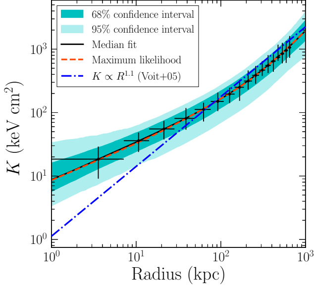
Figure 3. The entropy profile for SPT0607, computed from the derived density profile and an isothermal temperature profile. The analytic profile has been discretized in the same binning scheme used to fit the emission measure data. We find a low entropy core and good agreement in the cluster outskirts with the expected K \propto R^{1.1} relation from Voit et al. (2005).
