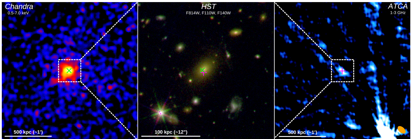
Figure 1. Left: Merged Chandra X-ray counts image in the broad-band 0.5–7.0 keV. The image is binned such that each pixel is 0''.984 on each side and then smoothed with a Gaussian kernel of 4 pixels. The green “x” shows the location of the X-ray peak, which we use as the center for all X-ray profiles. Middle: RGB image of SPT0607 using the HST F140W (red), F110W (green), F814W (blue) filters. The green “x” shows the location of the X-ray peak and the magenta “+” shows the location of the radio peak, both of which are coincident with the BCG of SPT0607. Right: ATCA 2 GHz radio image with the synthesized beam in orange in the lower right corner. The magenta “+” shows the location of the radio peak.
