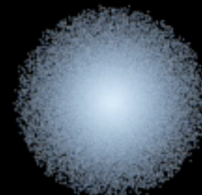
Disk 180K Halo 1M
